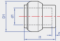
Sizes 15 - 28mm
