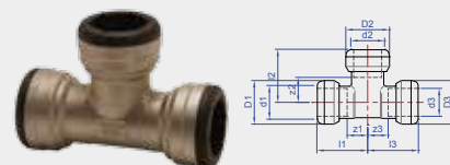
Sizes 35 - 54mm
