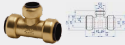
Sizes 22 - 28mm
