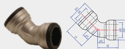
Sizes 35 - 54mm
