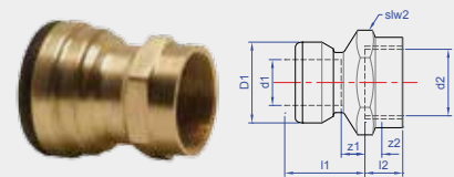
Sizes 35 - 54mm
