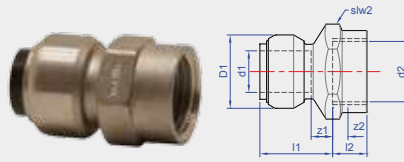
Sizes 15 - 28mm
