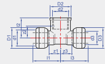
Sizes 35 - 42mm
