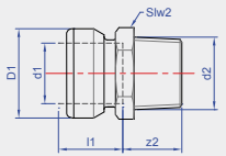
Sizes 35 - 54mm
