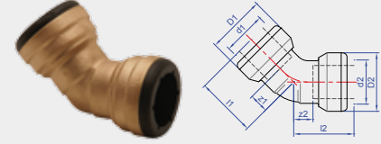
Sizes 35 - 54mm
