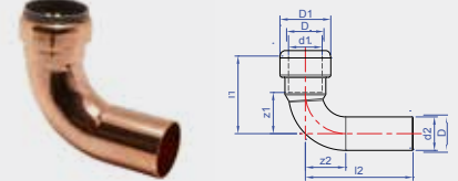
Sizes 35 - 54mm
