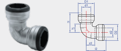
Sizes 35 - 54mm
