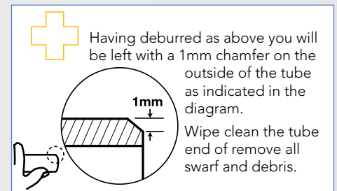
Remove burrs
