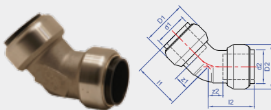
Sizes 15 - 28mm
