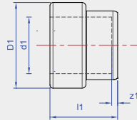
Sizes 15 - 28mm
