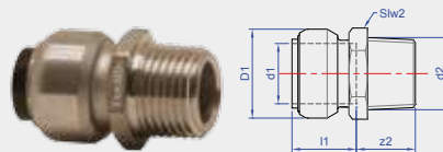
Sizes 15 - 28mm
