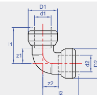
Sizes 35 - 54mm
